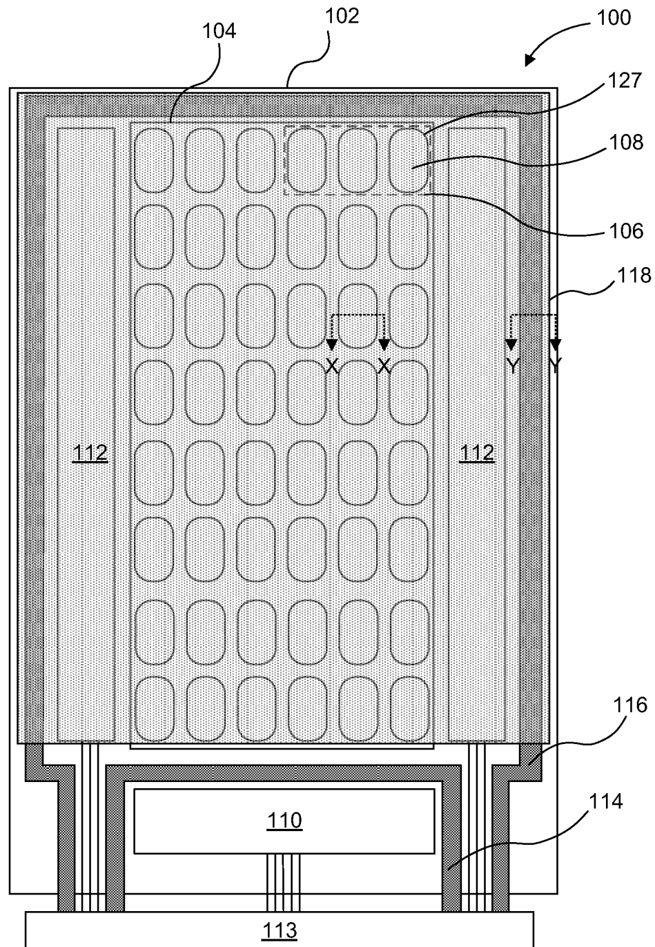
FIG. 1 PRIOR ART
