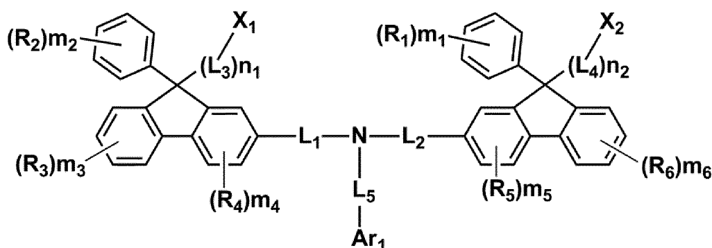
[Chemical Formula 1]
