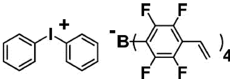
[Chemical Formula 8]
