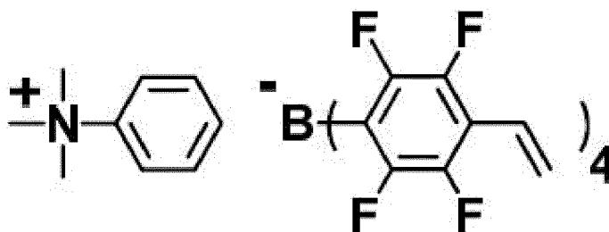
[Chemical Formula 9]
