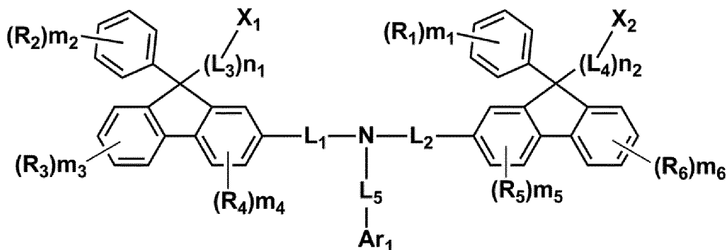
[Chemical Formula 1]
