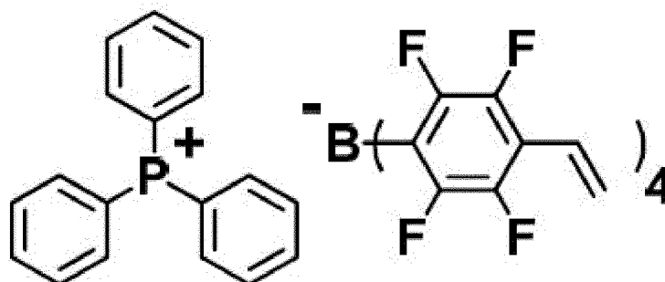
[Chemical Formula 9]
