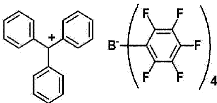
[Chemical Formula 5]
