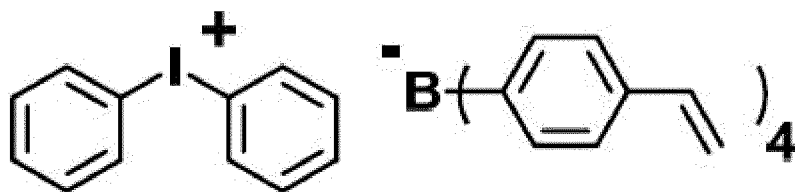
[Chemical Formula 7]
