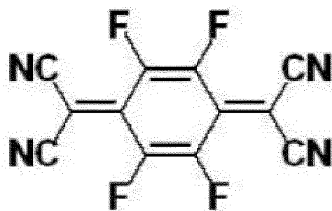
[Chemical Formula 3]
