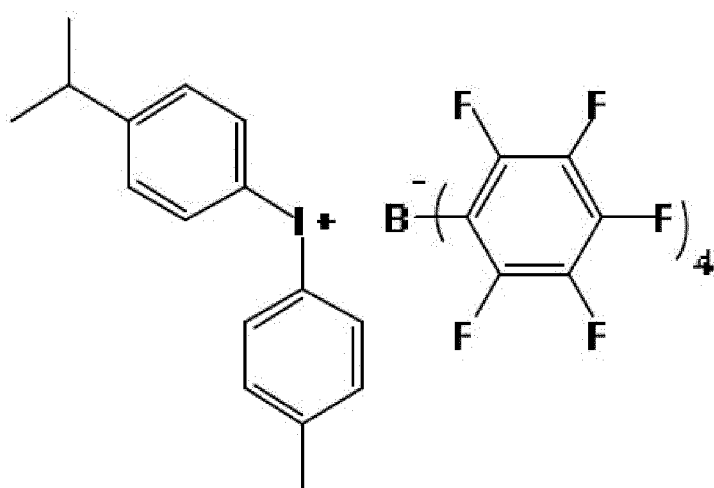
[Chemical Formula 5]
