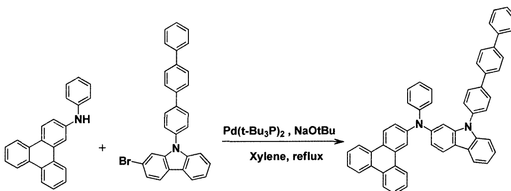
[Compound A]
