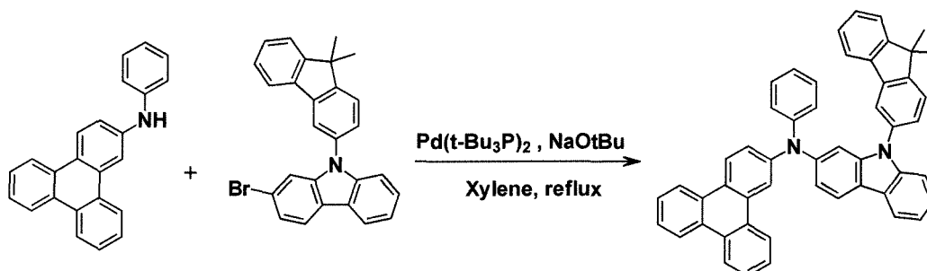
[Compound A]
