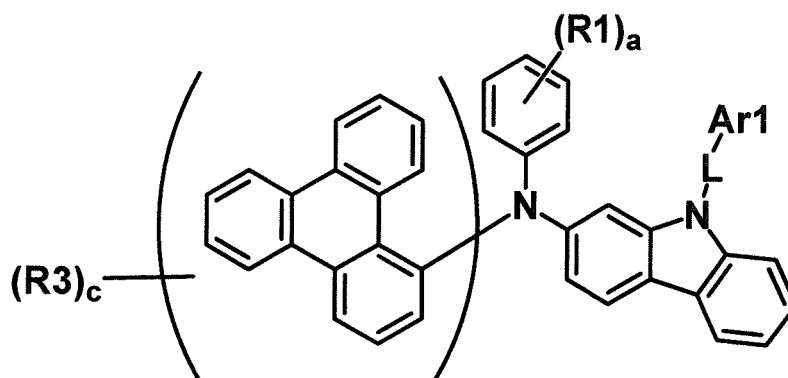
[Chemical Formula 3]
