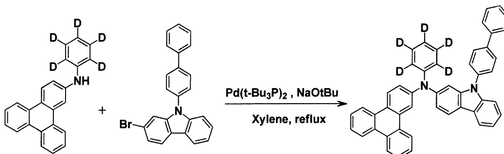
[Compound F]
