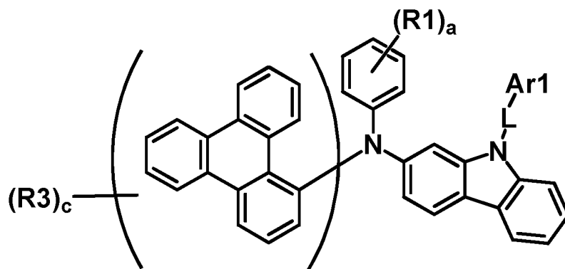
[Chemical Formula 3]
