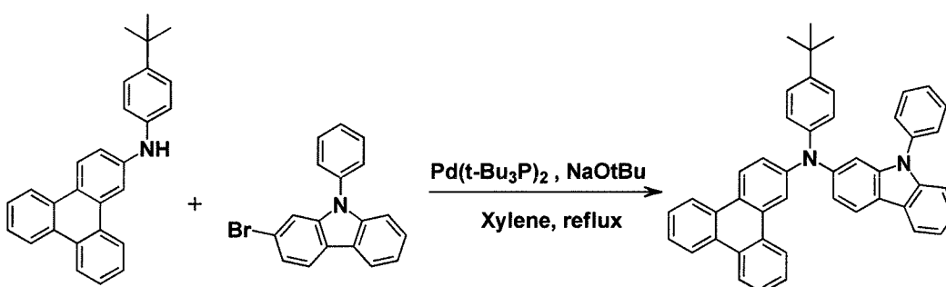
[Compound D]
