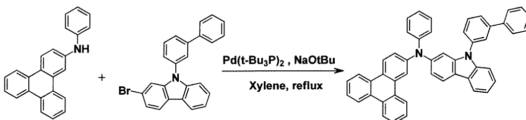
[Compound A]
