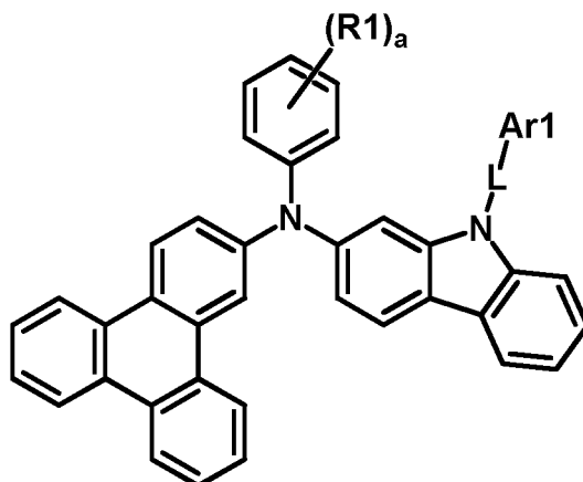
[Chemical Formula 4]
