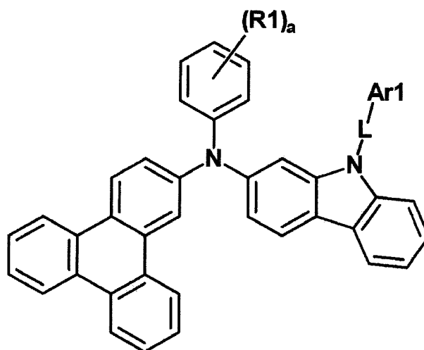
[Chemical Formula 5]
