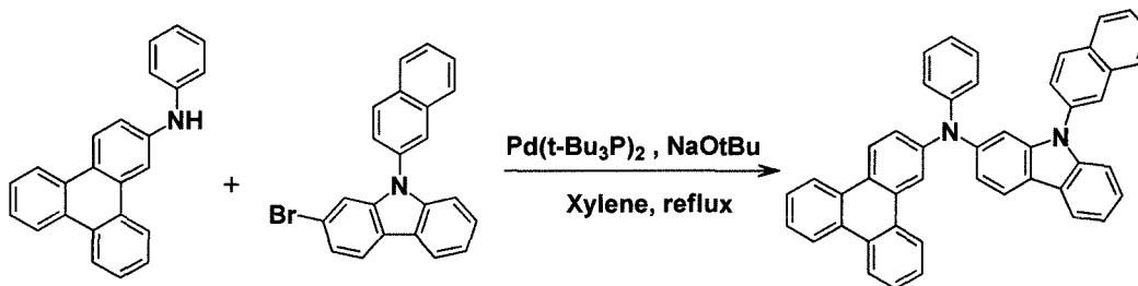
[Compound A]
