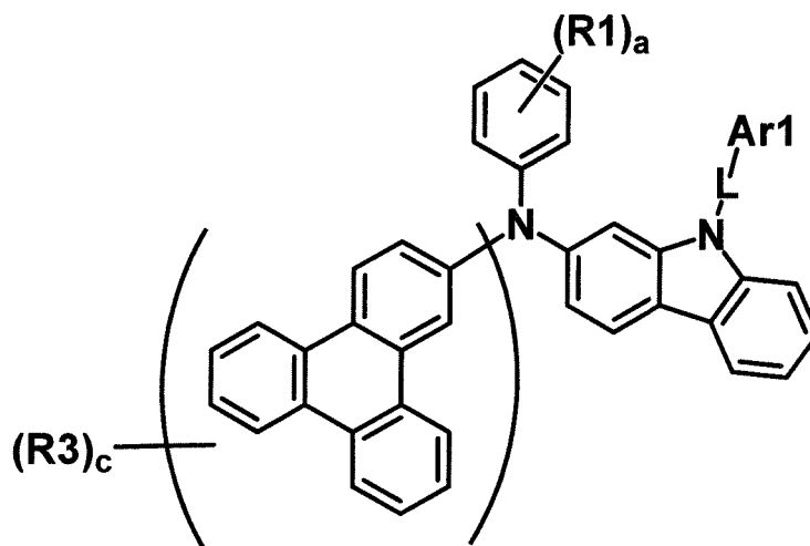
[Chemical Formula 2]
