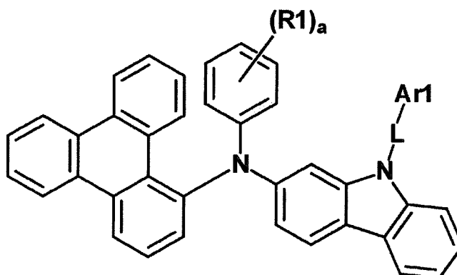
[Chemical Formula 5]
