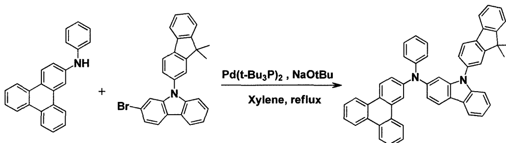
[Compound A]
