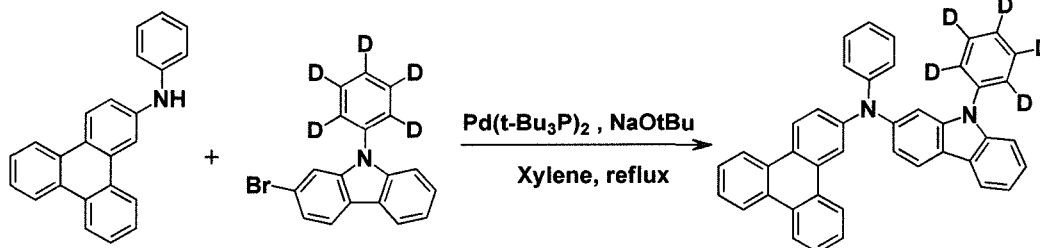
[Compound A]
