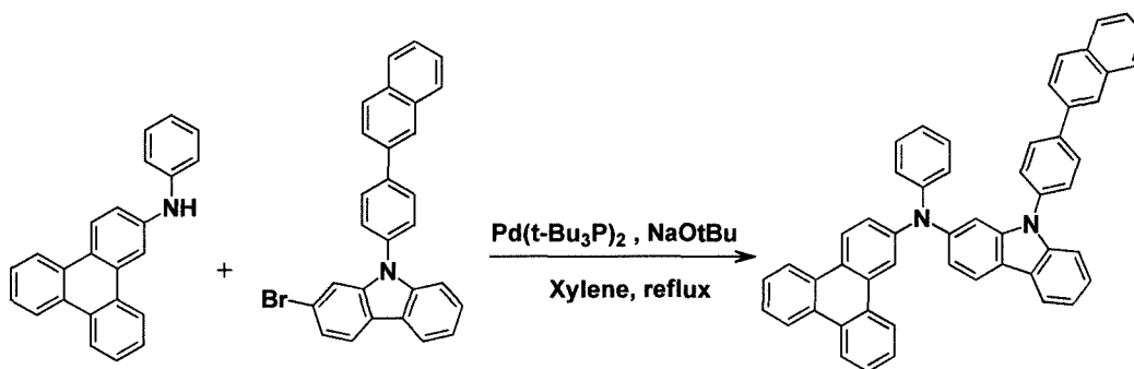
[Compound A]
