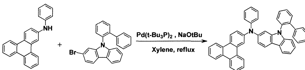
[Compound A]
