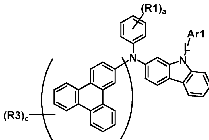
[Chemical Formula 3]
