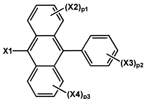
[Chemical Formula 7]
