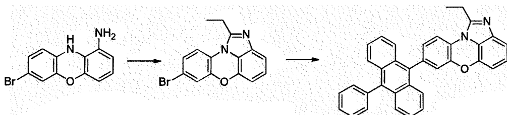
[Compound 1-C]
