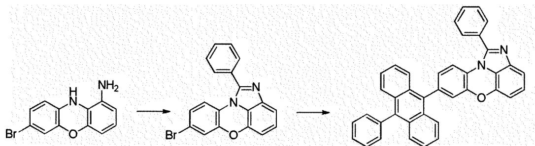
[Compound 1-C]
