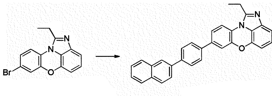
[Compound 2-A]
