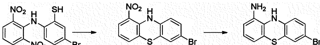
[Compound 2-1-A]
