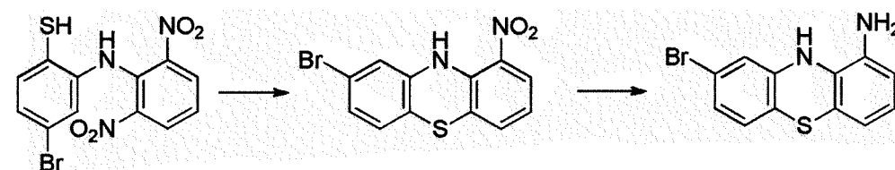
[Compound 2-2-A]
