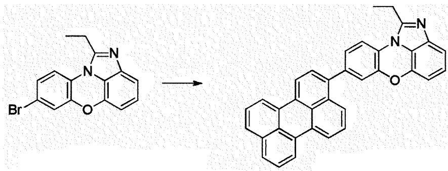
[Compound 2-A]
