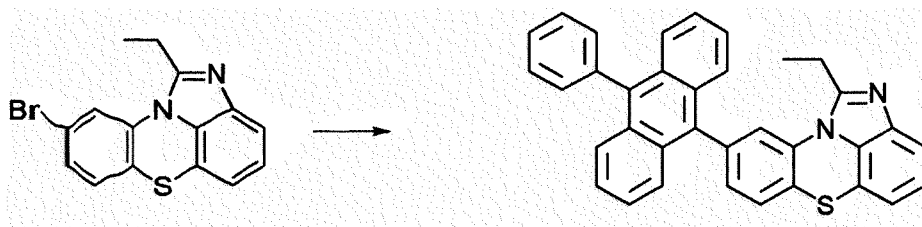
[Compound 2-2-D]
