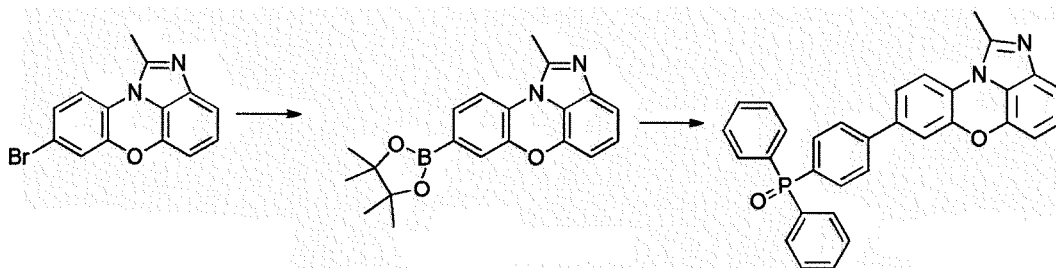
[Compound 1-D]
