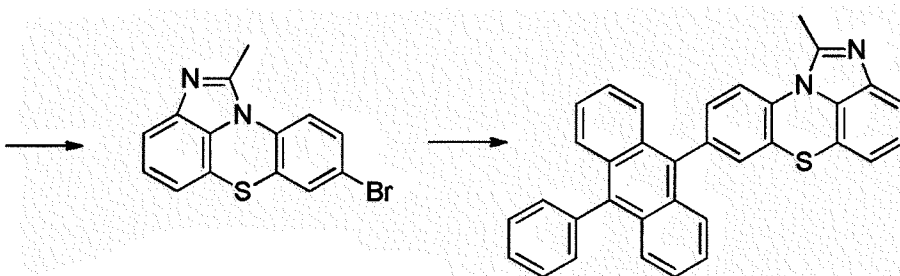
[Compound 2-1-D]
