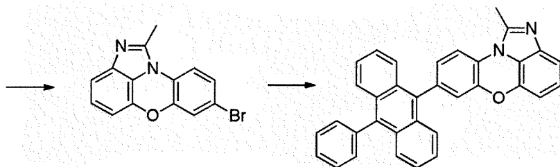
[Compound 1-D]
