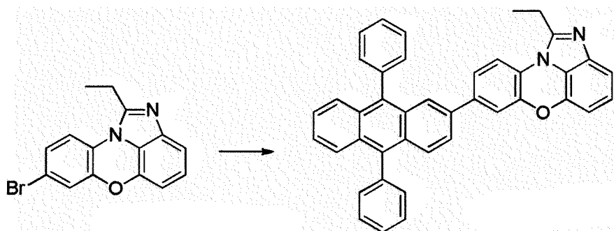
[Compound 2-A]
