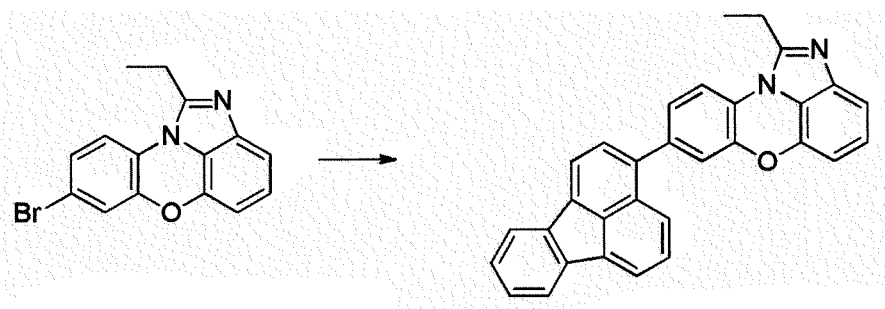
[Compound 2-A]
