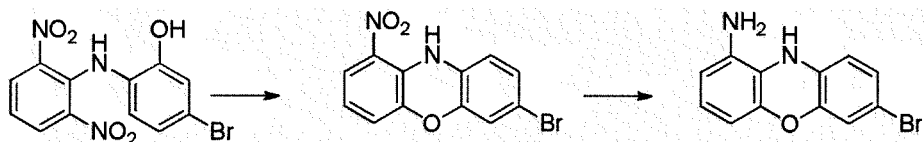
[Compound 1-A]
