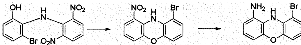
[Compound 18-A]
