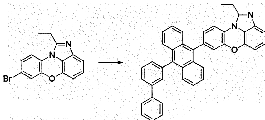
[Compound 2-A]
