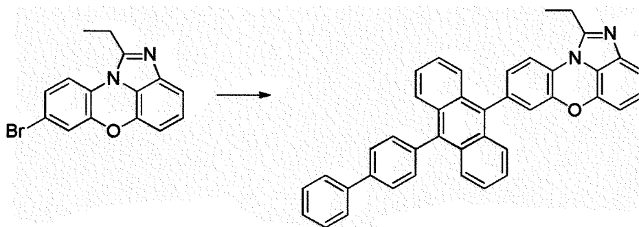
[Compound 2-A]
