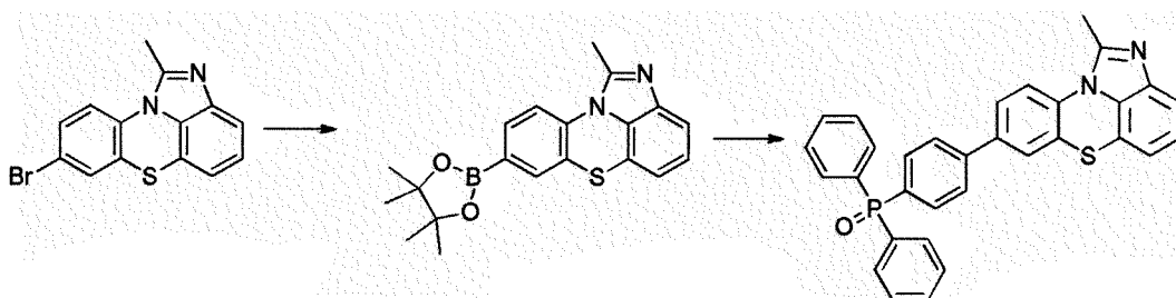
[Compound 2-1-D]
