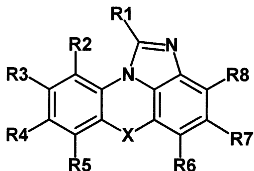
[Chemical Formula 3]
