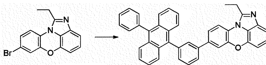
[Compound 2-A]
