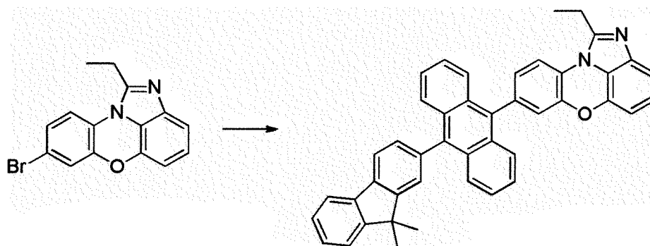
[Compound 2-A]
