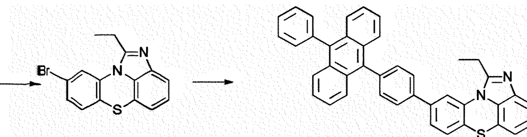
[Compound 2-2-D]
