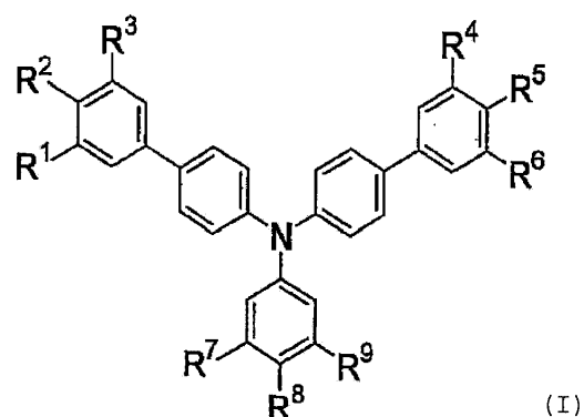
[Chem 1]
