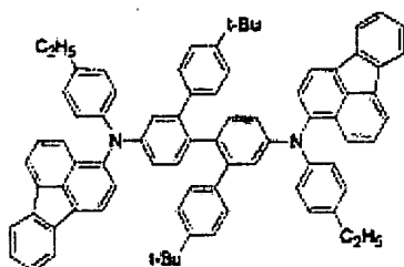
Structural Formula (F12)
