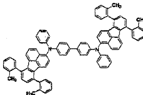
Structural Formula (F14)
