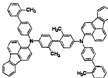
Structural Formula (F11)
