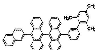
Structural Formula (A10)
