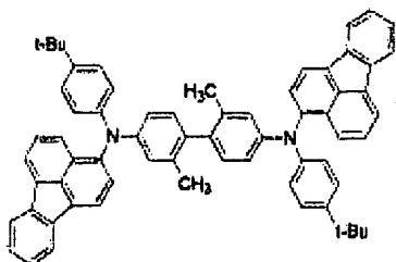
Structural Formula (F10)
