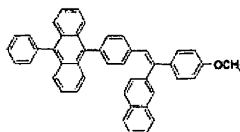
Structural Formula (A6)
