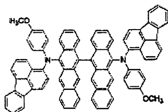
Structural Formula (F19)
