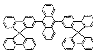
Structural Formula (A8)
