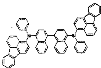
Structural Formula (F15)
