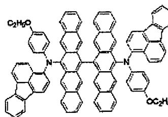
Structural Formula (F20)
