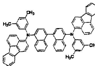
Structural Formula (F16)
