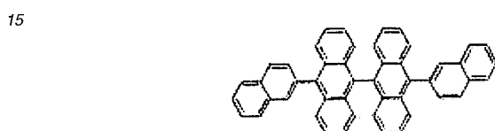
Structural Formula (A9)
