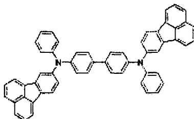
Structural Formula (F21)
