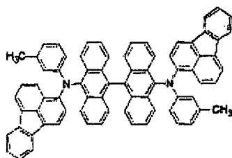
Structural Formula (F17)
