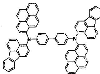
Structural Formula (F8)
