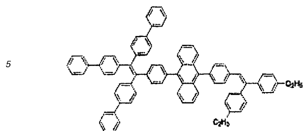
Structural Formula (A7)
