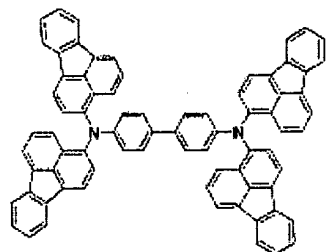
Structural Formula (F7)
