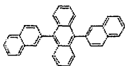
Structural Formula (A1)
