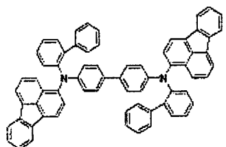
Structural Formula (F9)
