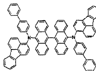
Structural Formula (F18)
