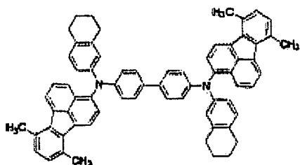
Structural Formula (F13)
