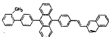
Structural Formula (A3)
