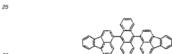
Structural Formula (A11)
