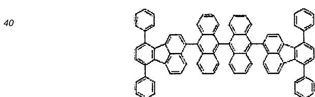
Structural Formula (A13)
