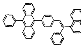
Structural Formula (A4)
