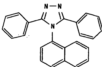
25 3-phenyl-4-(1-naphthyl)-5-phenyl-1,2,4-triazole
