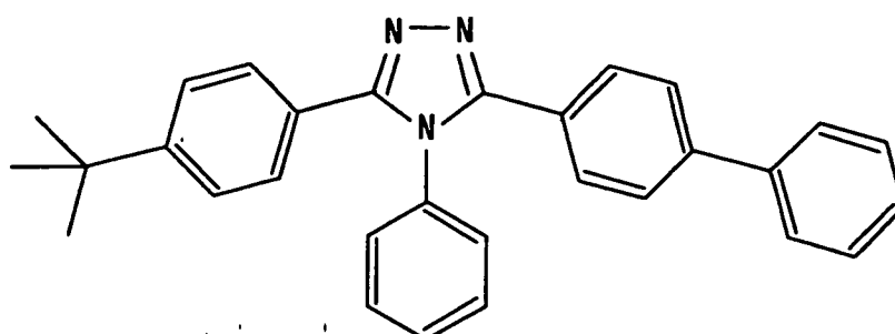
45 3-(4-tert-butylphenyl)-4-phenyl-5-(4'-biphenyl)-1,2,4-triazole
