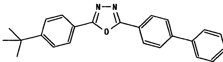
10 2-(4-tert-butylphenyl)-5-(4-biphenyl)-1,3,4-oxadiazole
