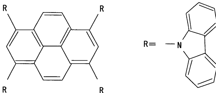
Structural formula (15)
