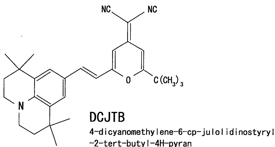
Structural formula (14)
