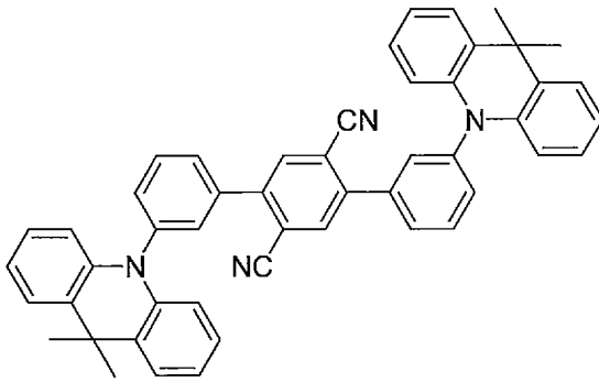
Compound 11
