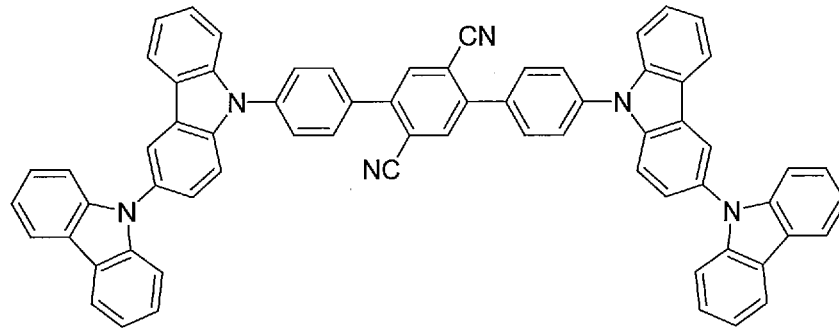
Compound 5
