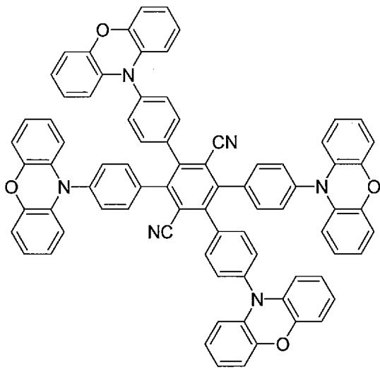
Compound 9
