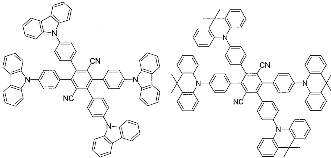
Compound 7
