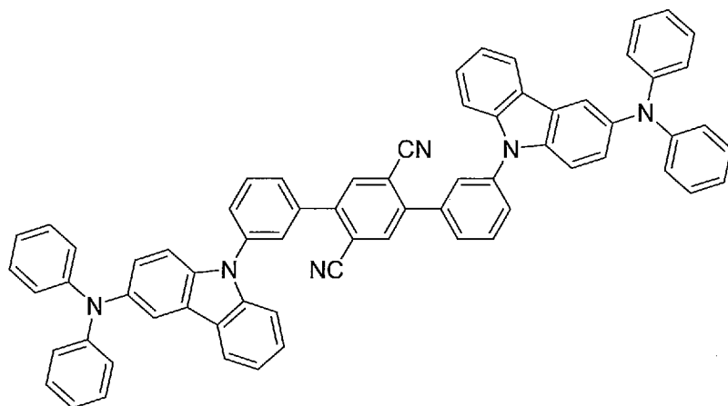
Compound 14
