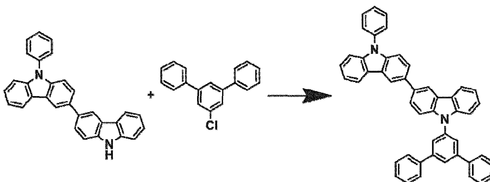
[Chemical Formula 27]
