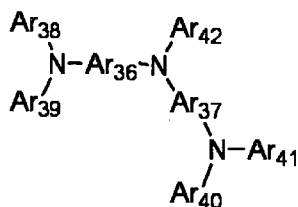
General formula [14]
