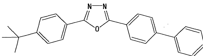
2-(4-tert-butylphenyl)-5-(4-biphenyl)- -1,3,4-oxadiazole
