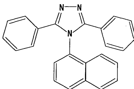
3-phenyl-4-(1-naphthyl)- -5-phenyl-1,2,4-triazole
