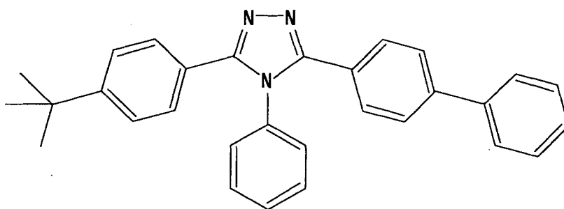
3-(4-tert-butylphenyl)-4-phenyl -5-(4'-biphenyl)-1,2,4-triazole
