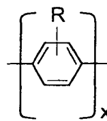
PPP derivatives
