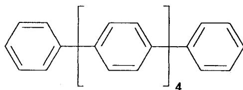
p-sexiphenyl
