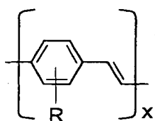
PPV derivatives
