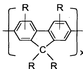
PF derivatives
