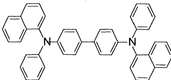
NPD
