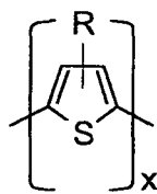
PAT derivatives
