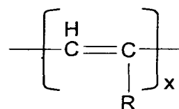
PA derivatives
