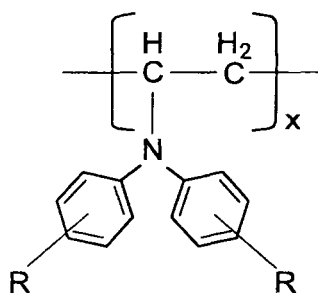
PVCz derivatives
