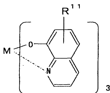
Structural formula (3)
