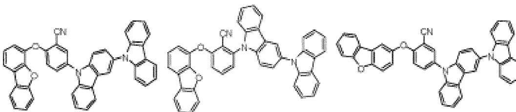
compound 1
