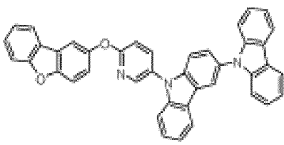
compound 7
