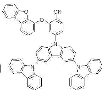
compound 17
