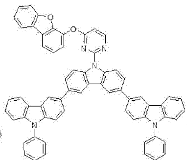
compound 23
