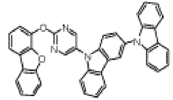
compound 9
