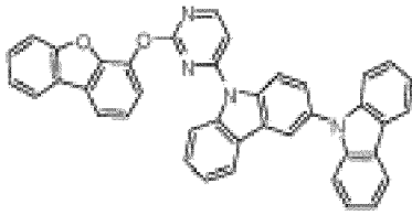
compound 10
