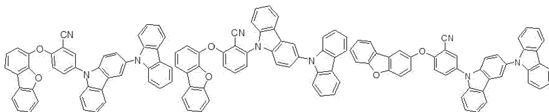
compound 1
