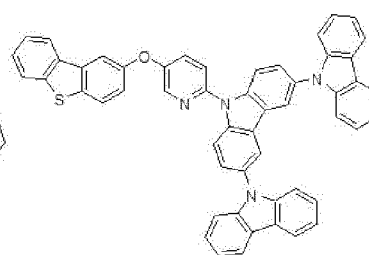
compound 21
