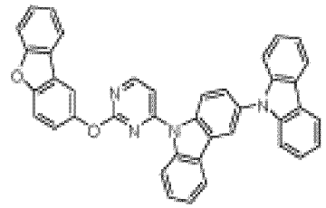
compound 12
