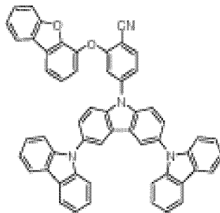
compound 17
