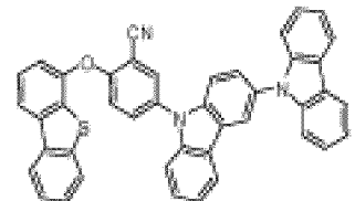
compound 15
