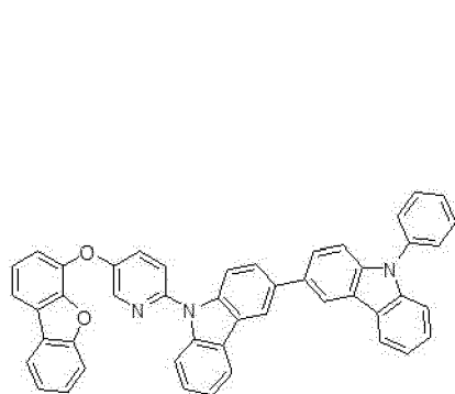
compound 19
