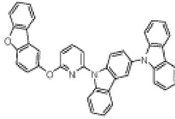
compound 8
