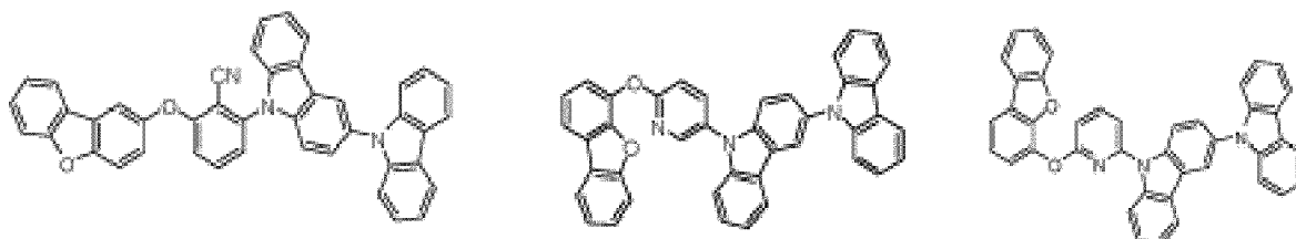
compound 4
