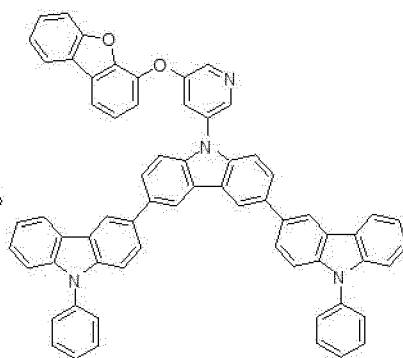
compound 20
