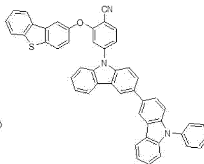
compound 18
