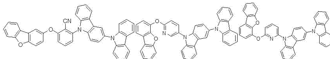
compound 4
