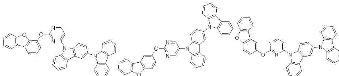
compound 10
