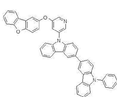
compound 22
