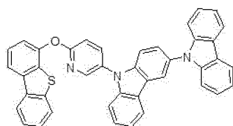
compound 16
