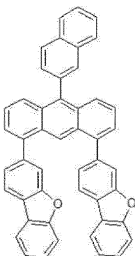
[Chemical formula 3]
