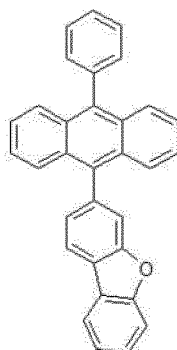
[Chemical formula 1]
