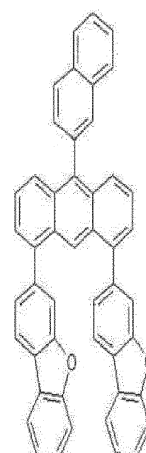
[Chemical formula 3]
