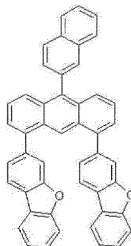
[Chemical formula 3]
