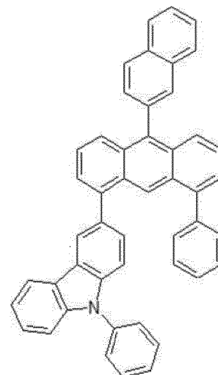
[Chemical formula 6]
