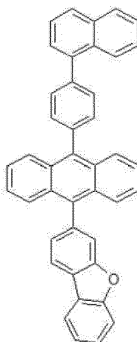
[Chemical formula 2]
