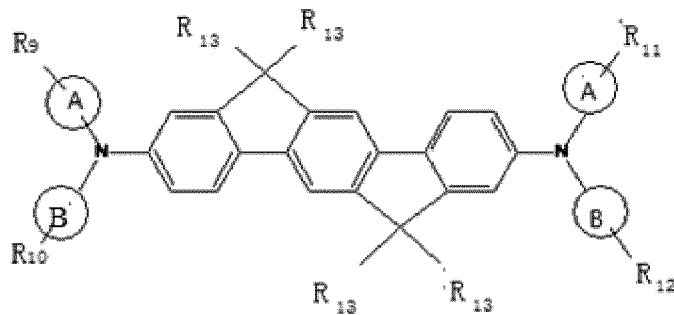
structural formula (3)
