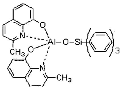
SAIq
