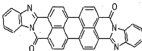
Perylene-based compound
