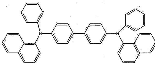
alpha-NPD
