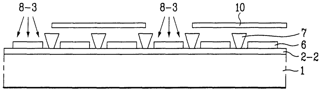
FIG. 2A Related Art
