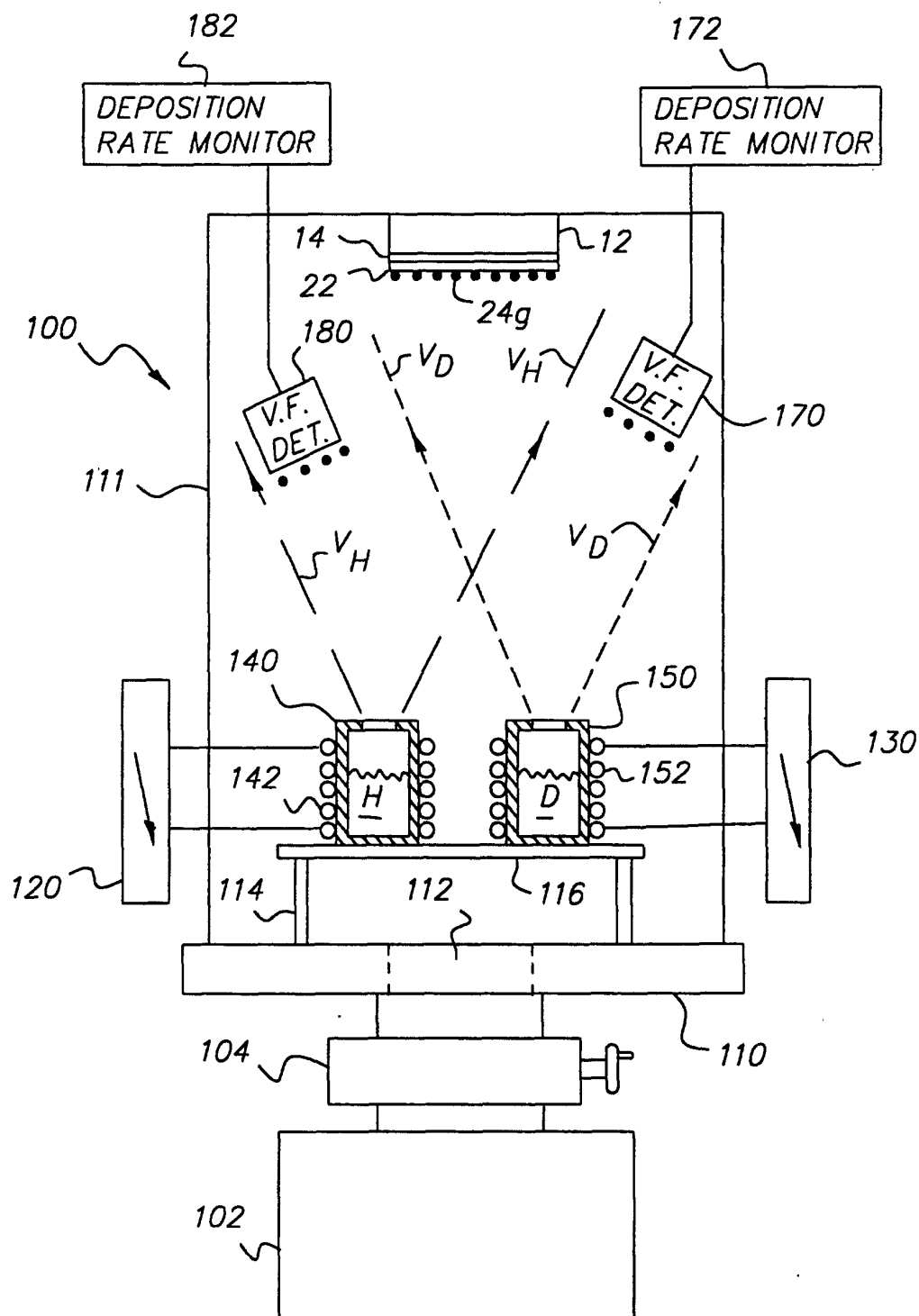
FIG. 2 (PRIOR ART)
