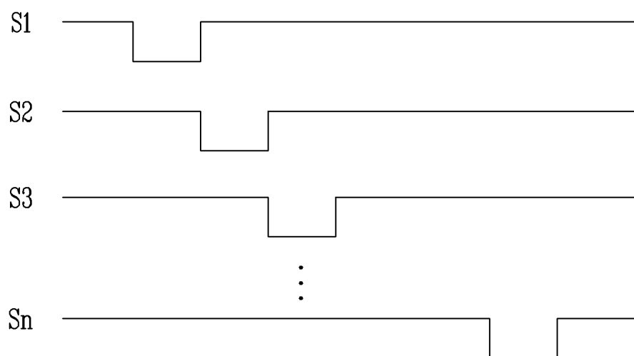
FIG. 2 (PRIOR ART)
