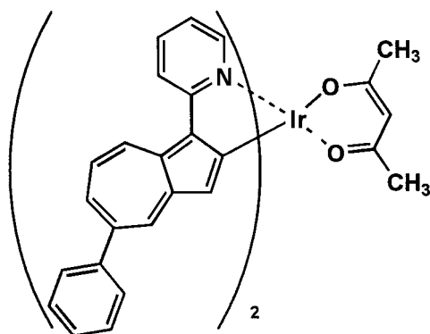
5-5
