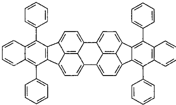
TPDBP.
