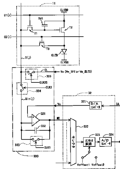
321 D/A converter 322 Selector 323 Offset circuit 324 A/D converter
