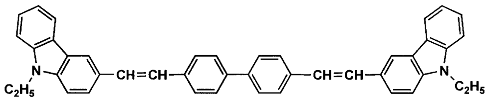
BCzVBi
