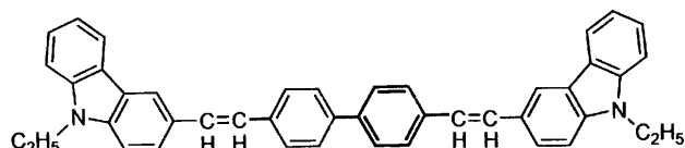
BCzVBi
