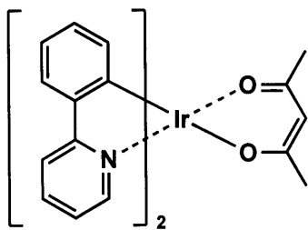
D-3(Ir(ppy) 3 )
