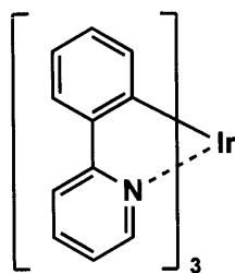
D-3(Ir(ppy) 3 )
