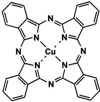
HT-1(CuPc)
