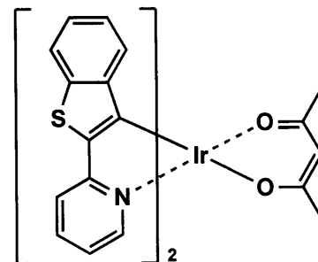
D-4(Btp 2 Ir(acac))
