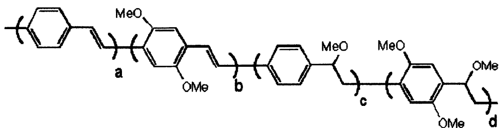
PPV copolymer
