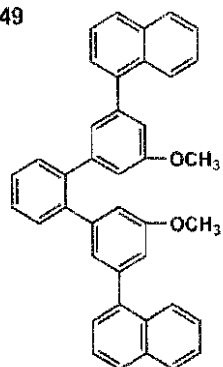
(I)-51
