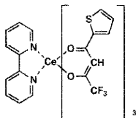
RE-12
