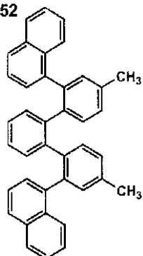
(I)-54
