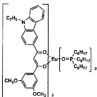
RE-20
