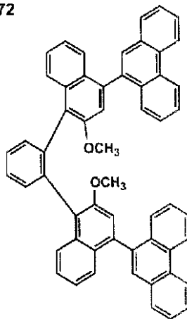
(I)-74
