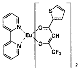
RE-11
