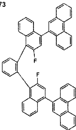
(I)-74
