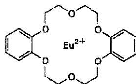
RE-5
