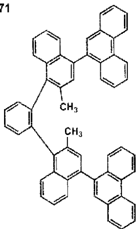
(I)-73
