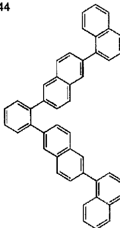
(I)-46
