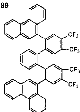
(I)-91
