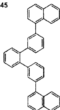
(I)-47
