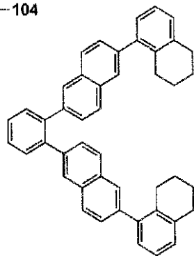
(I)-107
