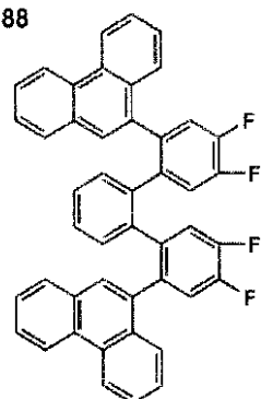
(I)-90
