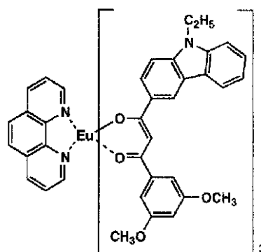
RE-19
