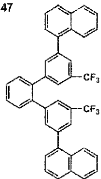
(I)-47
