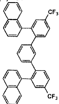
(II)-57
