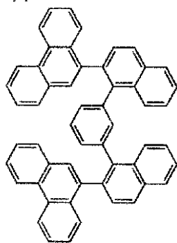
(II)-74
