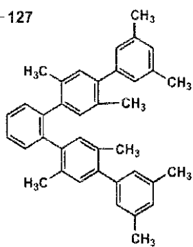
(I)-129
