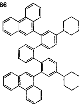
(I)-88
