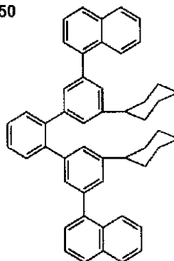
(I)-52
