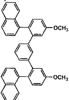
(II)-60
