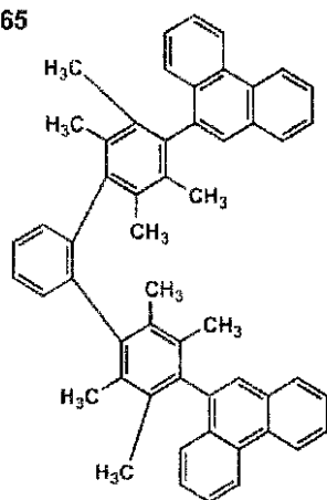
(I)-66
