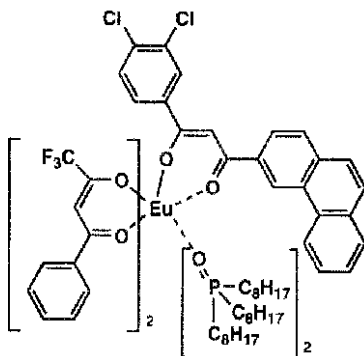
RE-18
