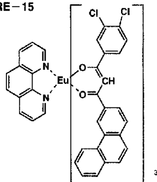
RE-15
