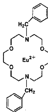
RE-7
