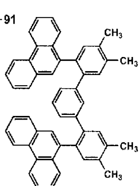
(II)-94
