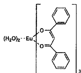
RE-16
