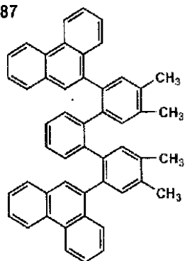
(I)-89
