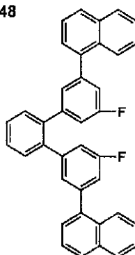
(I)-48
