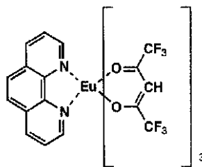
RE-14
