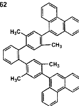
(I)-64
