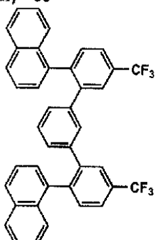
(II)-61
