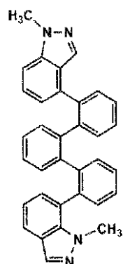
(I)-122
