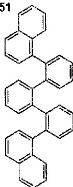
(I)-53
