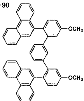
(II)-92
