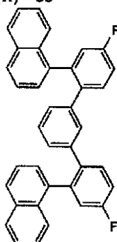
(II)-58
