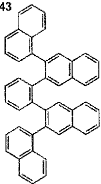
(I)-43
