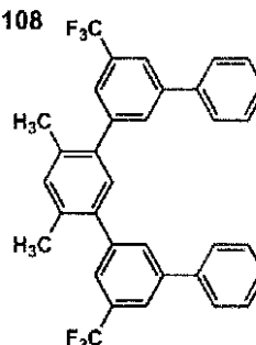
(II)-110
