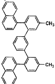
(II)-60
