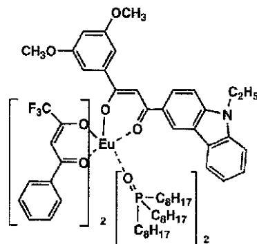
RE-21
