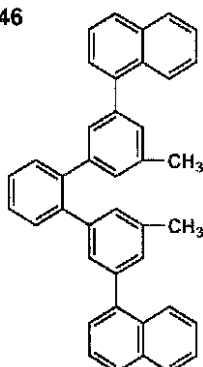
(I)-48
