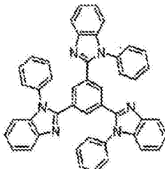
TPBi
