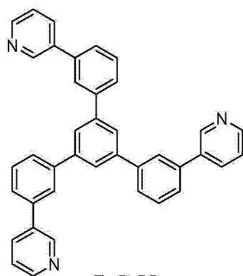
TmPyPB
