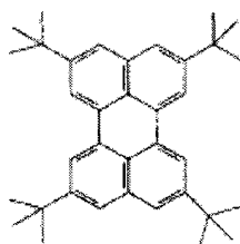
TBP
