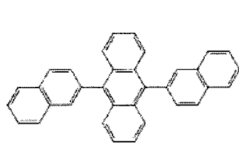
ADN
