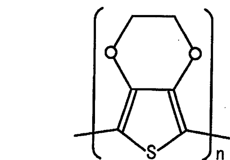
PEDOT ..... 聚-3,4-亚乙二氧基噻吩
