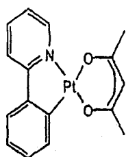
(ppy)Pt(acac)
