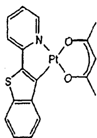
(btp)Pt(acac)
