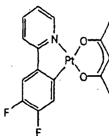
(4,5-F 2 ppy)Pt(acac)
