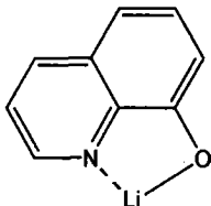
Liq
