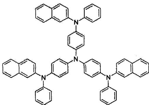
2-TNATA
