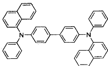
NPB
