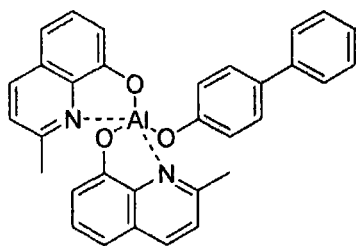
BAIq
