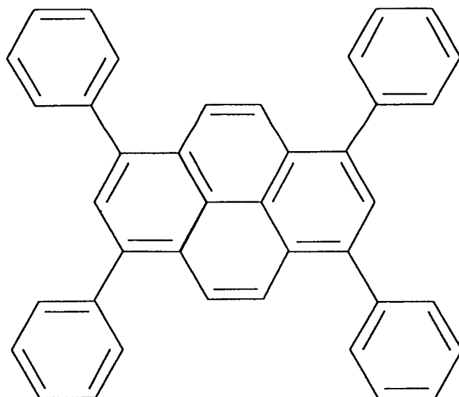
1,3,6,8-四苯基蒽
