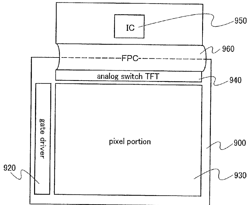
FIG. 17A IC connected by FPC
