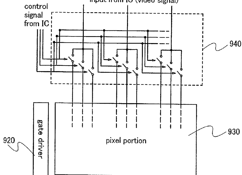
FIG. 17B IC formed by FPC, COG, and the like (switch portion) input from IC (video signal)
