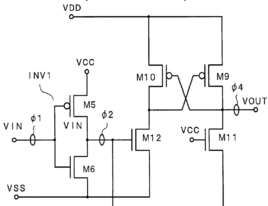
FIG. 14 (PRIOR ART)
