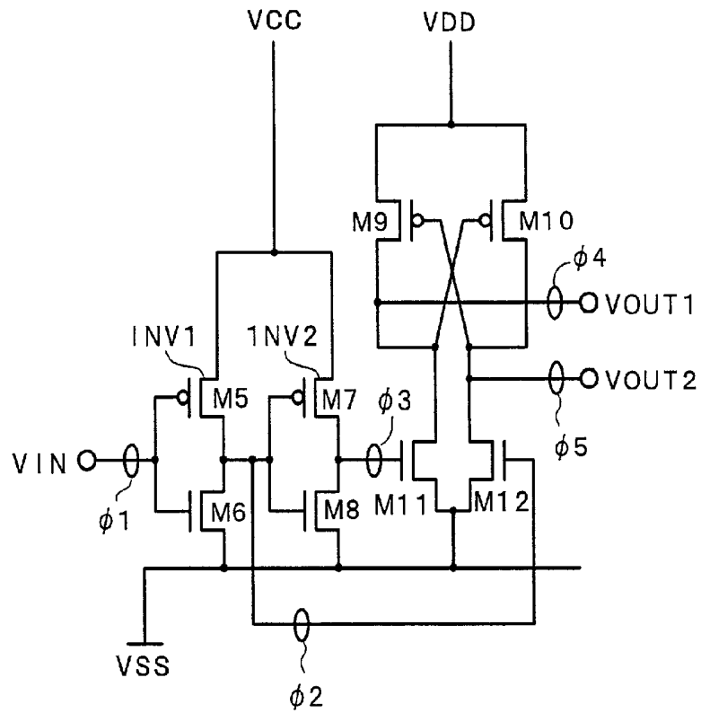
FIG. 14 (PRIOR ART)
