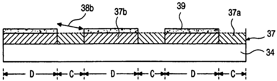
FIG. 2D (RELATED ART)
