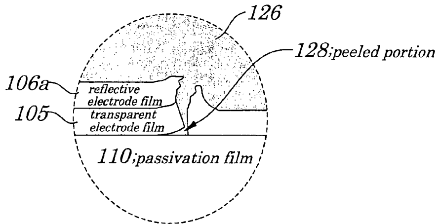
FIG. 31C(PRIOR ART)
