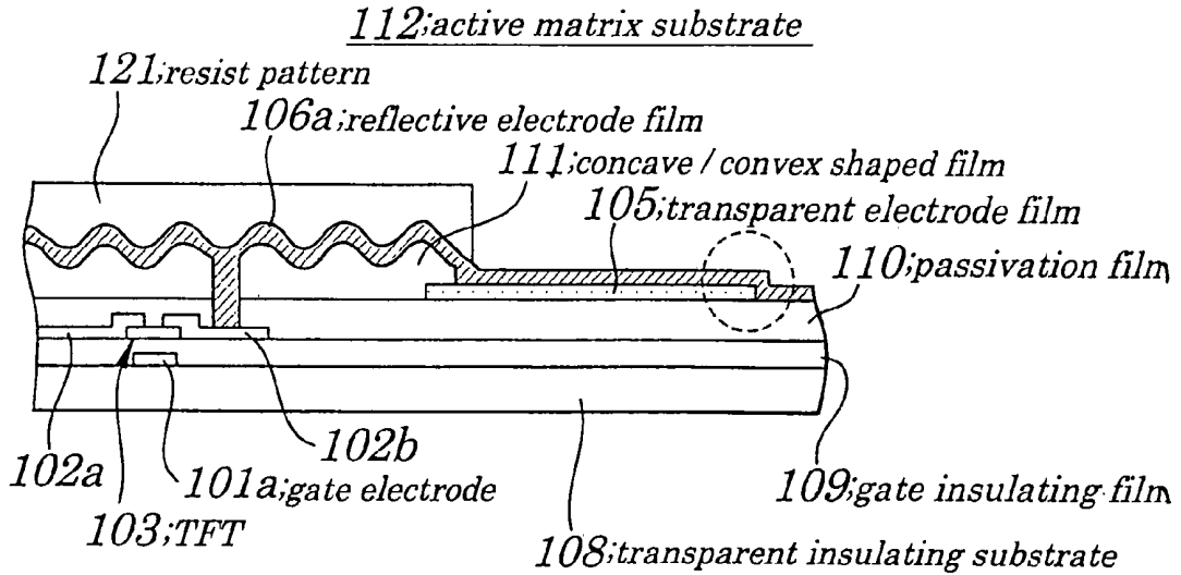
FIG. 31A(PRIOR ART)
