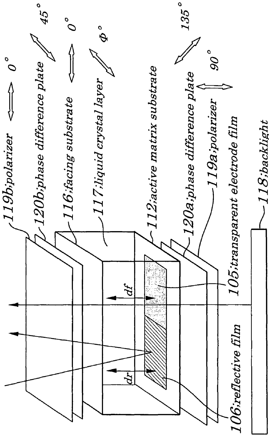
FIG. 34 (PRIOR ART)
