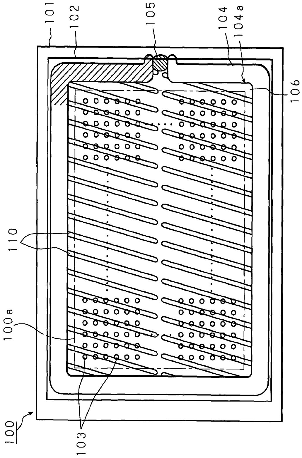
FIG. 1 PRIOR ART
