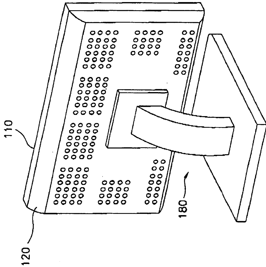
FIG. 3 (PRIOR ART)
