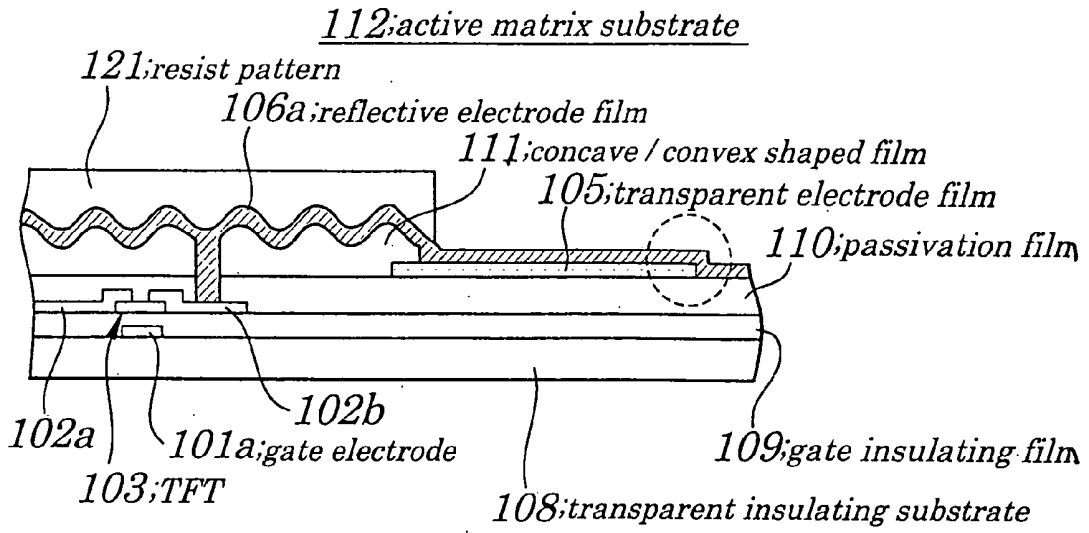
FIG. 31A(PRIOR ART)
