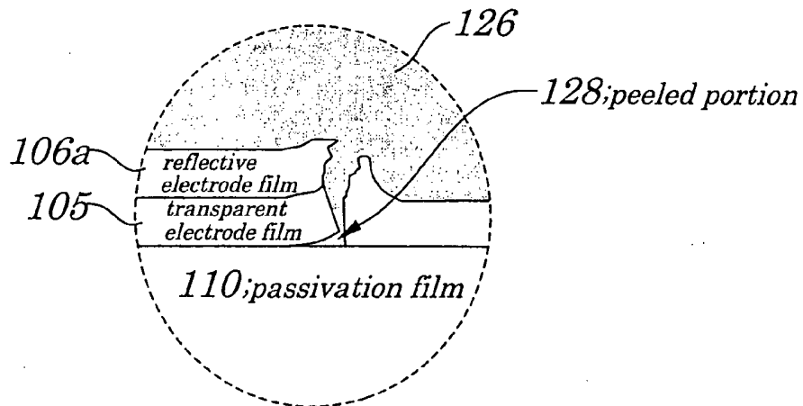
FIG. 31C(PRIOR ART)
