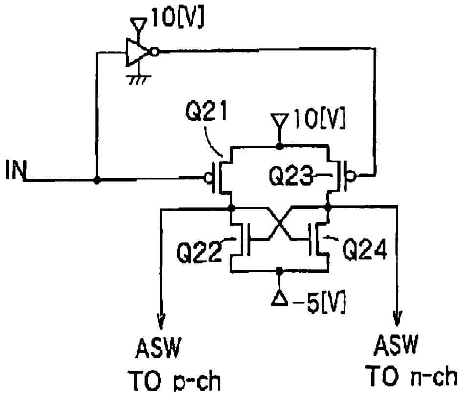
22: LEVEL CONVERSION CIRCUIT
