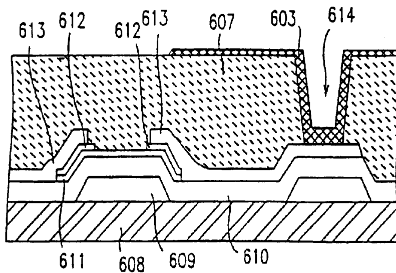
FIG. 38 (Prior Art)
