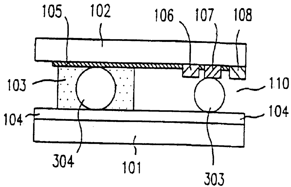
FIG. 36 (Prior Art)
