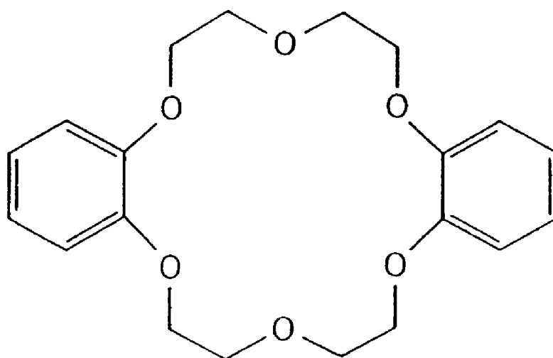
DIBENZOYL-18-CROWN-6
