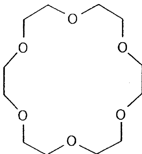
18-CROWN-6
