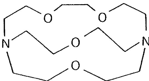
CRYPTAND [2.1.1]
