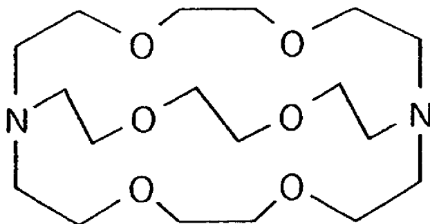
CRYPTAND [2.2.2]
