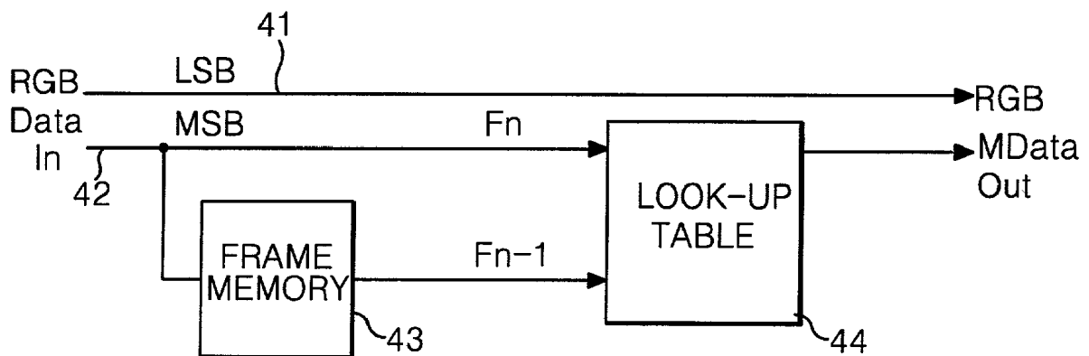
FIG. 4 CONVENTIONAL ART
