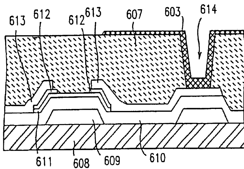
FIG. 38 (Prior Art)
