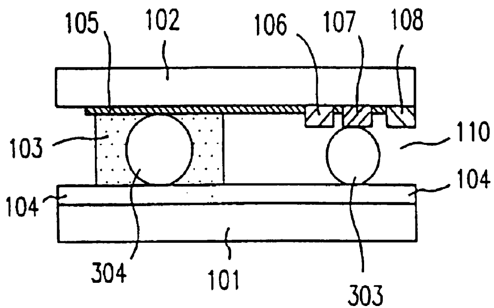
FIG. 36 (Prior Art)
