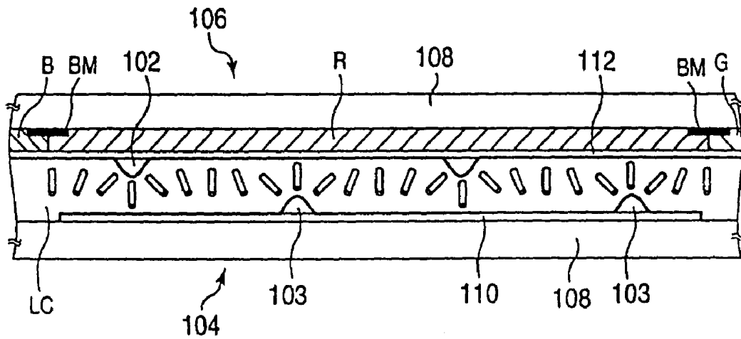
PRIOR ART FIG.37
