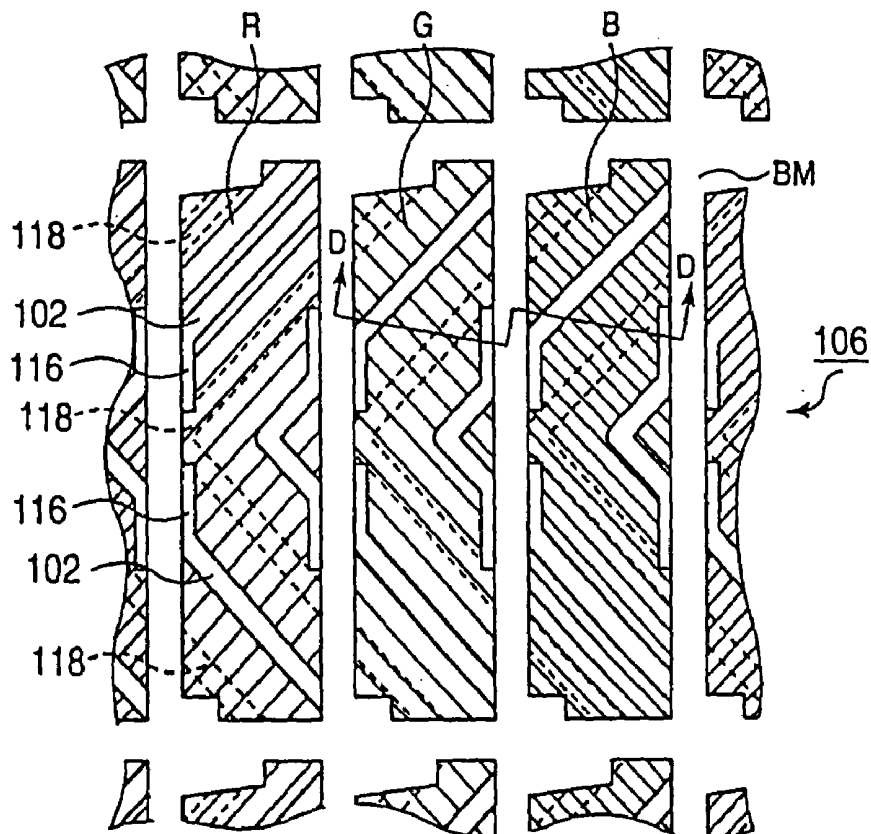
PRIOR ART FIG.41
