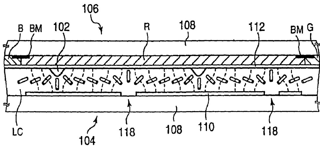
PRIOR ART FIG.39
