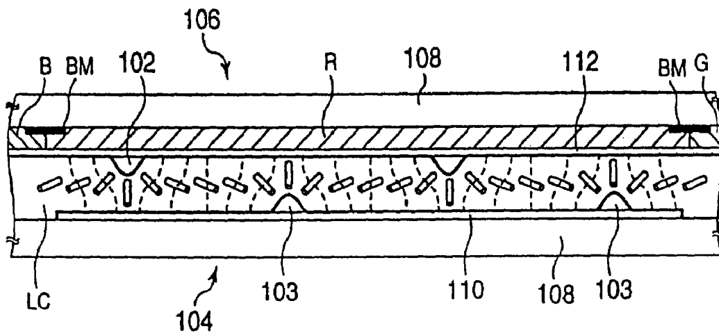
PRIOR ART FIG.38
