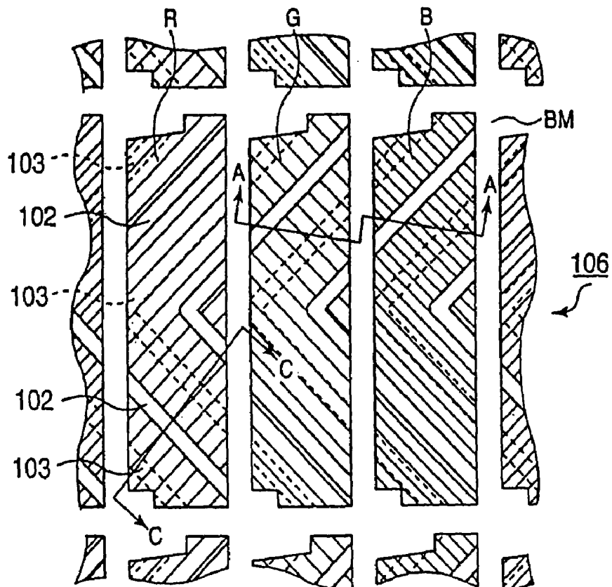
PRIOR ART FIG.35
