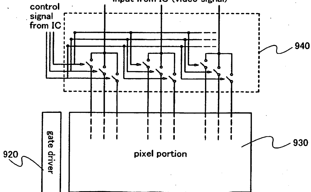
FIG. 17B IC formed by FPC, COG, and the like (switch portion) input from IC (video signal)
