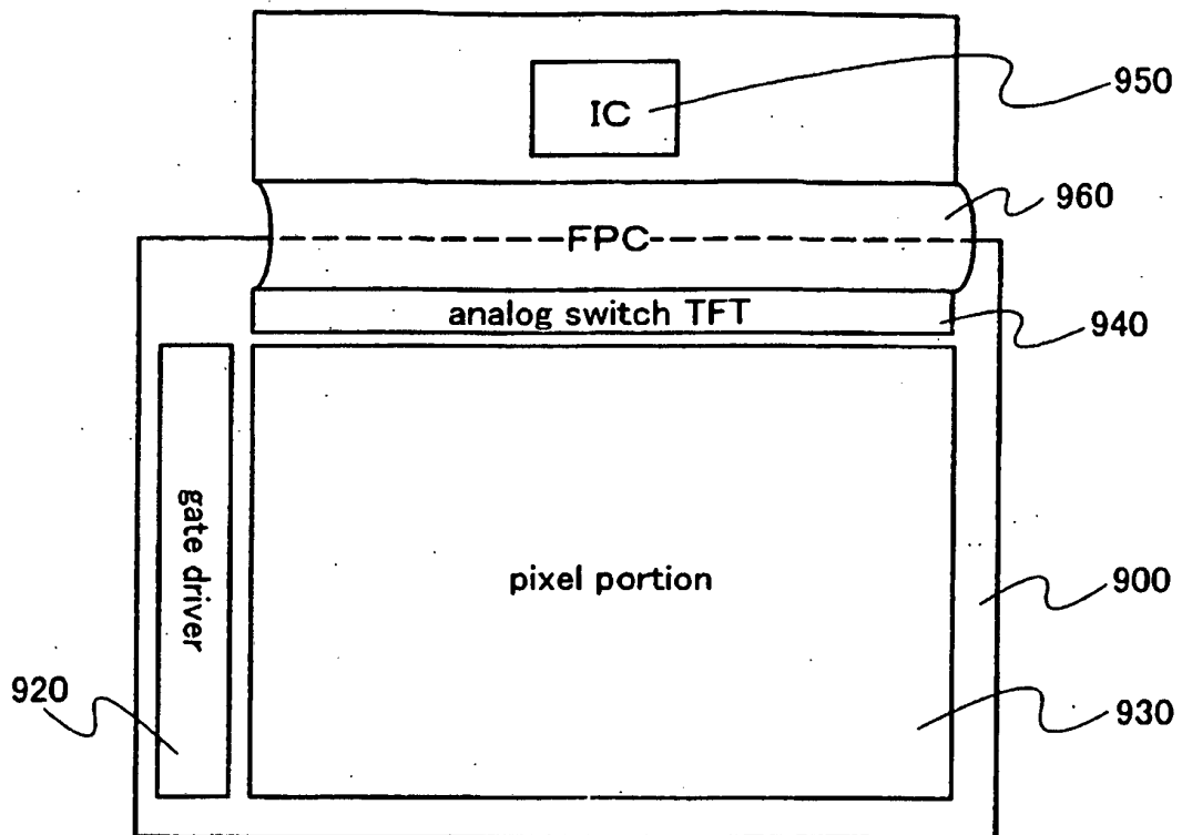
FIG. 17A IC connected by FPC
